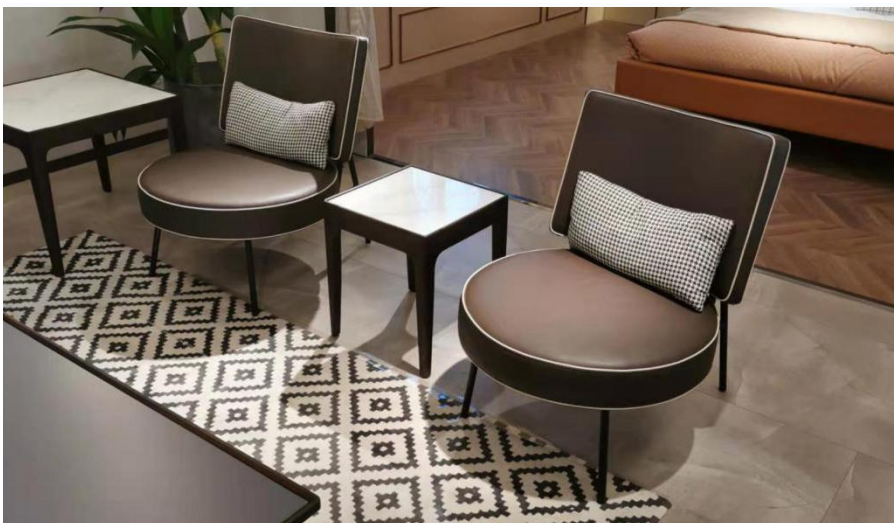
46#single chair
